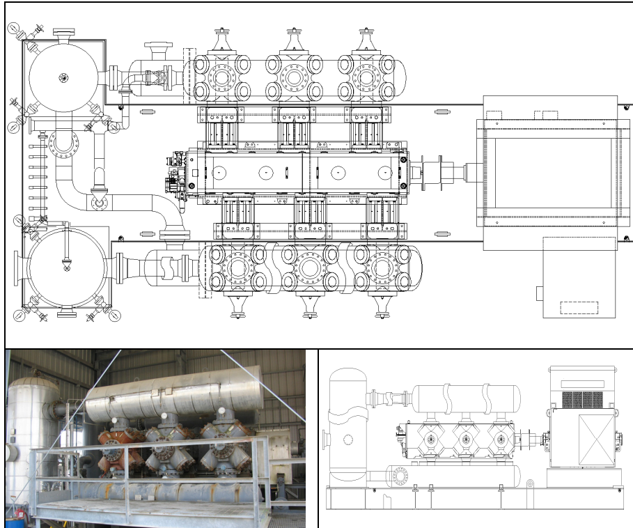
Figure 3: Compressor Plan and Elevation Views
