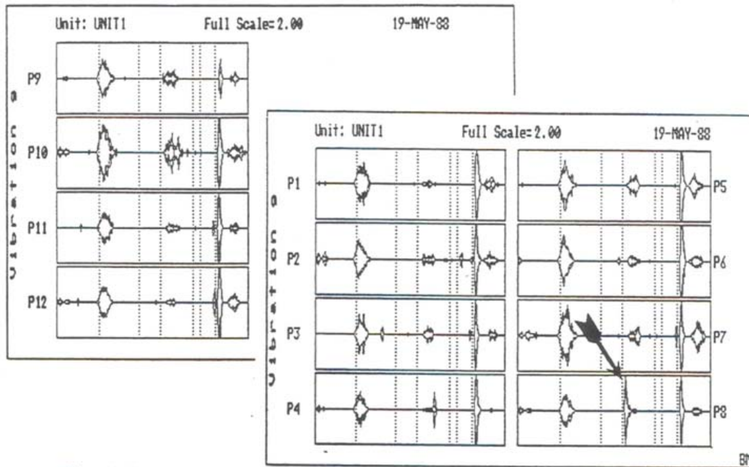
Figure 11 – Power Cylinder Vibration Patterns are displayed in groups of 8 for easy comparison
