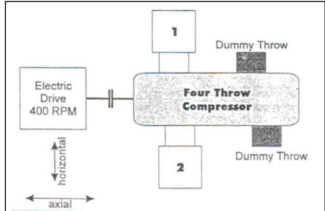
Figure 2 Rod and piston failures over many years made this unit uneconomic to run.
